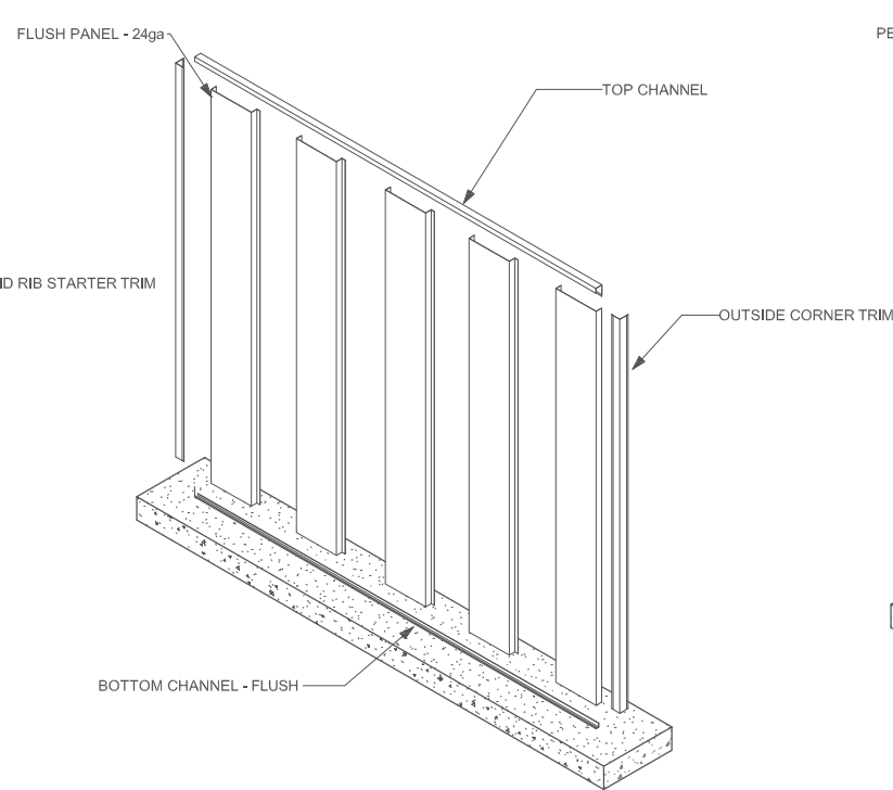
3 TYPICAL FLUSH PANEL ASSEMBLY
