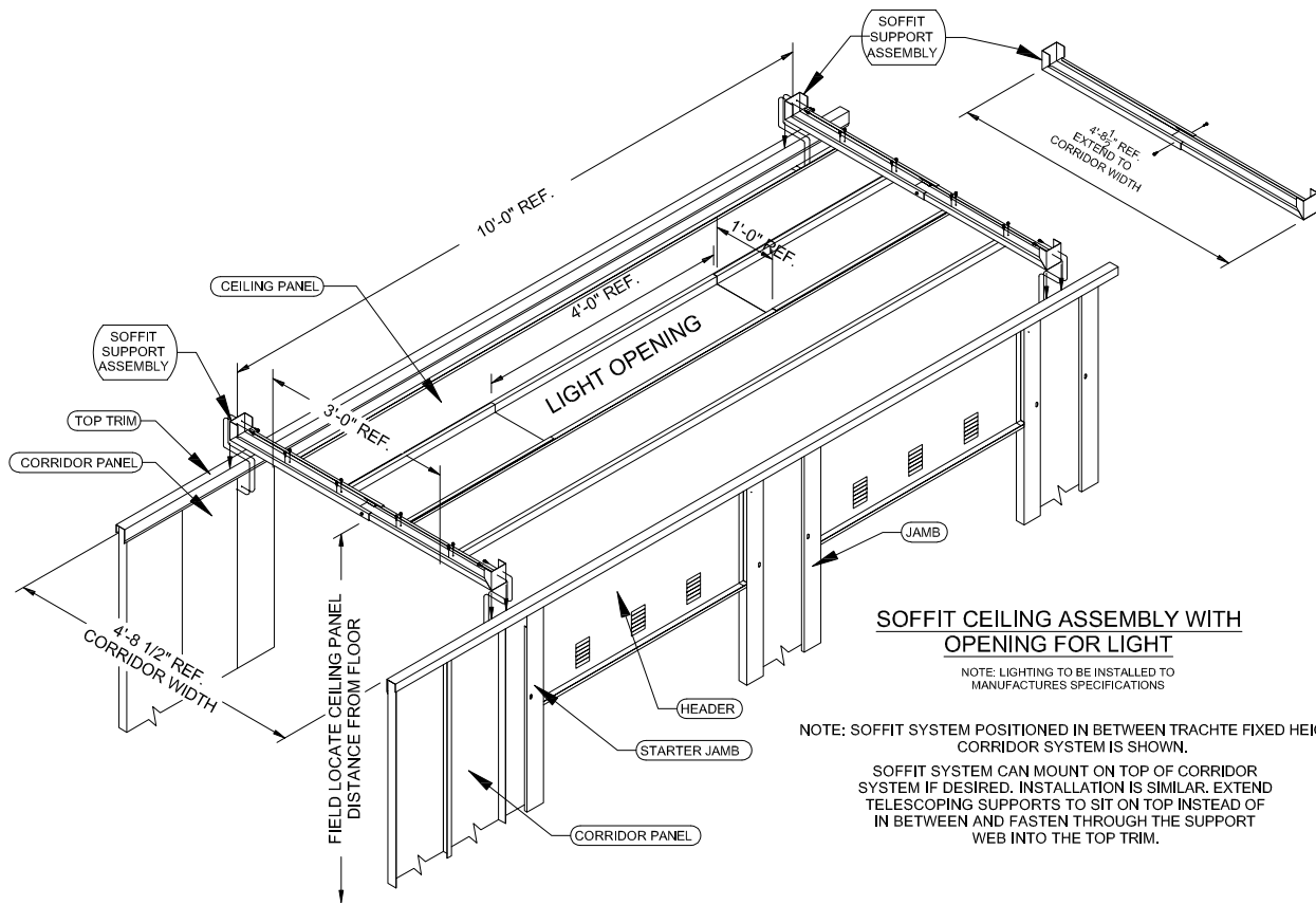
TYPICAL CORRIDOR SOFFIT CEILING PANEL OPTION DETAIL (WALL CONSTRUCTION MAY VARY)
