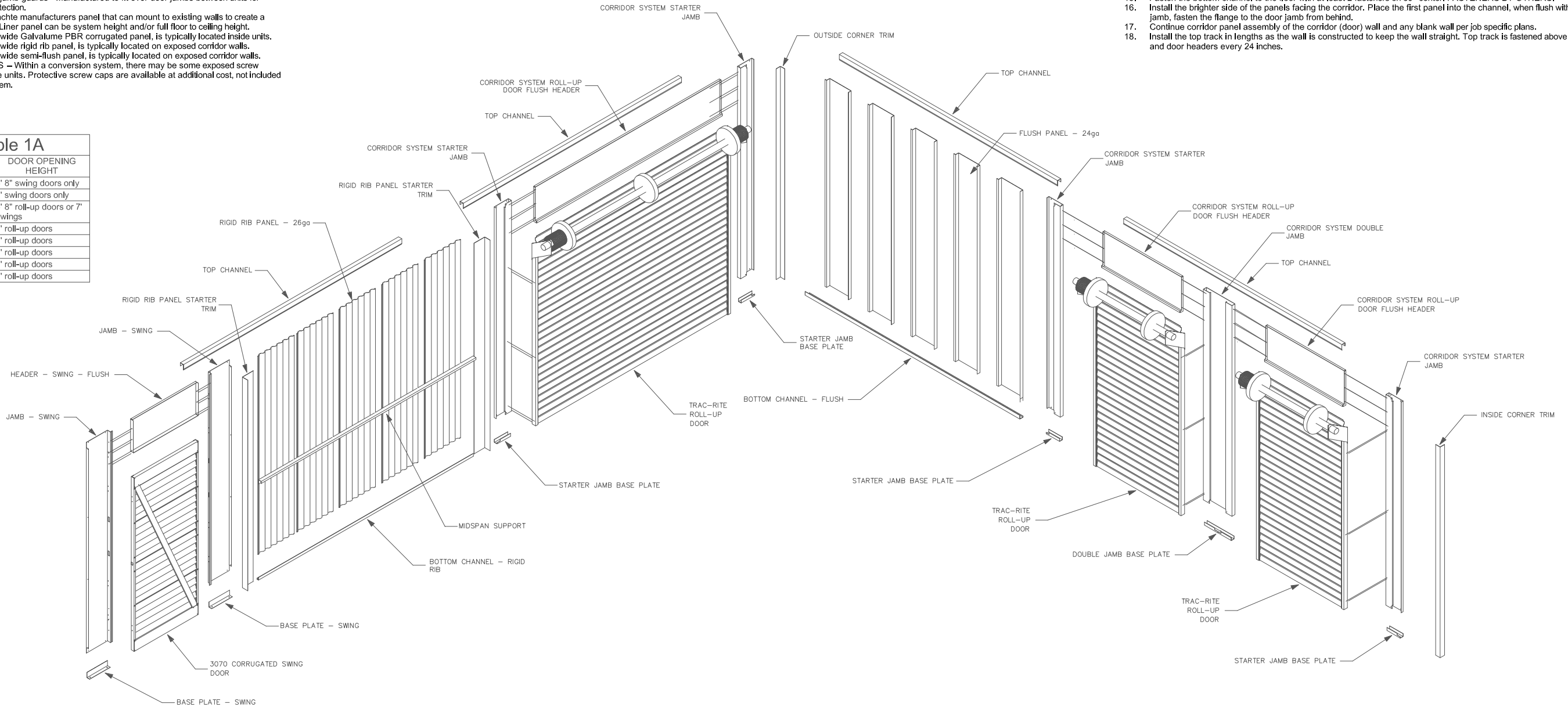
1 TRACHTE WALL CORNER
