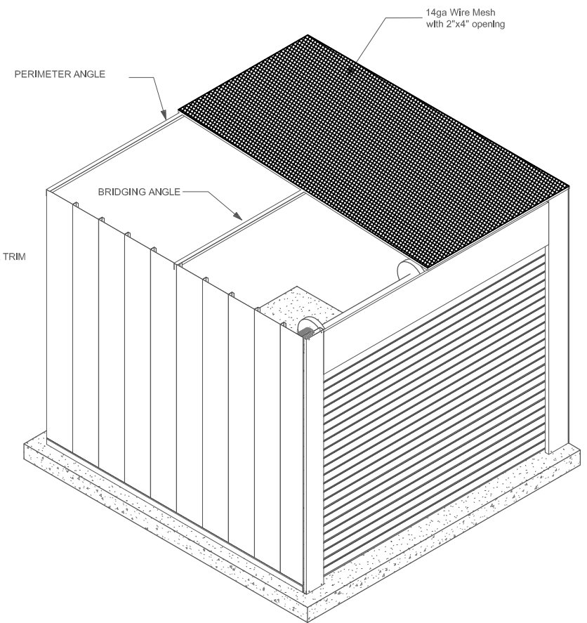
8 WIRE MESH SECURITY
