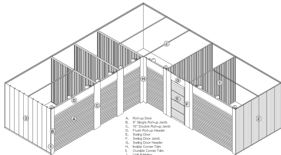
TYPICAL CONVERSION CORNER
