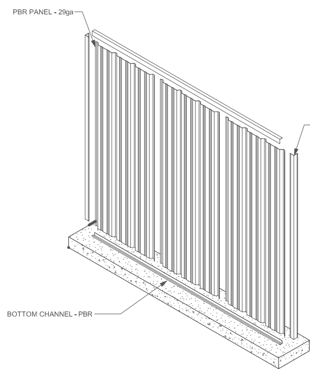
1 TYPICAL PBR PANEL ASSEMBLY
