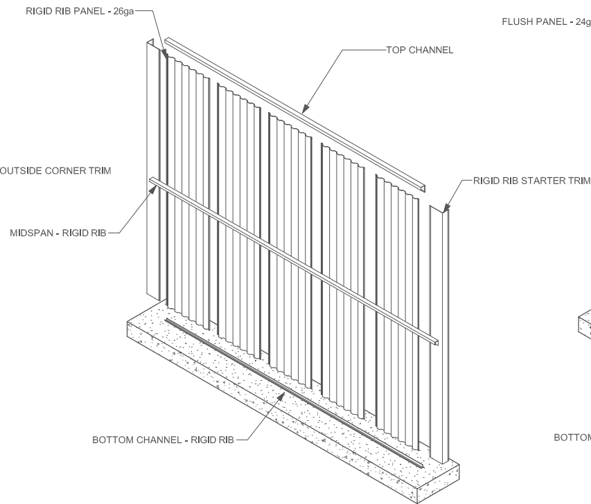
2 TYPICAL RIGID-RIB PANEL ASSEMBLY
